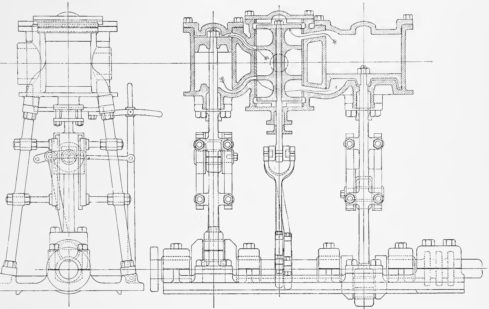
CHAPIN'S PATENT COMPOUND LAUNCH ENGINE.—Designed by John J. Chapin, Youkers, N. Y.
